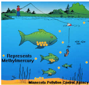
Bioaccumulation of Mercury (as methylmercury)
